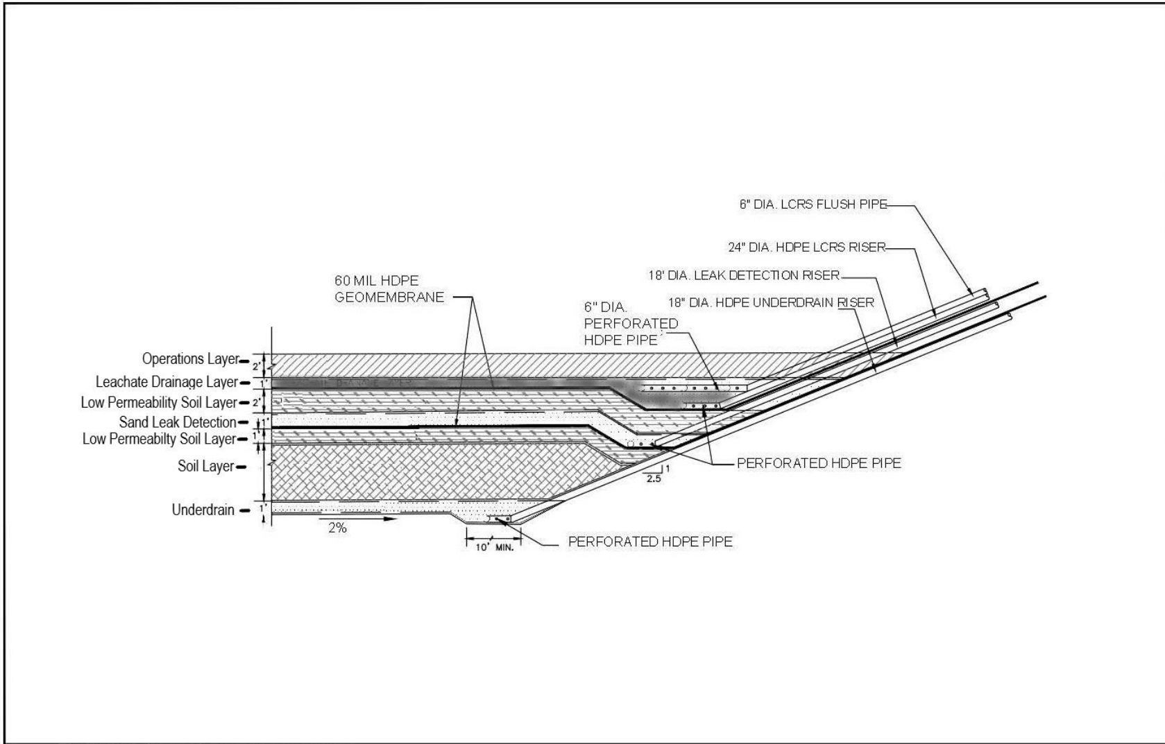
Phase IV LCRS and Underground Sumps Source SCS Engineers - Ameded Joint Technical Document, Central Disposal Site, Sonoma County, CA. Dated June 28, 2013
